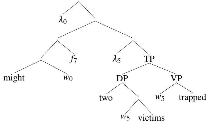
Figure 3 LF that derives the de dicto reading of (15), with world variables
