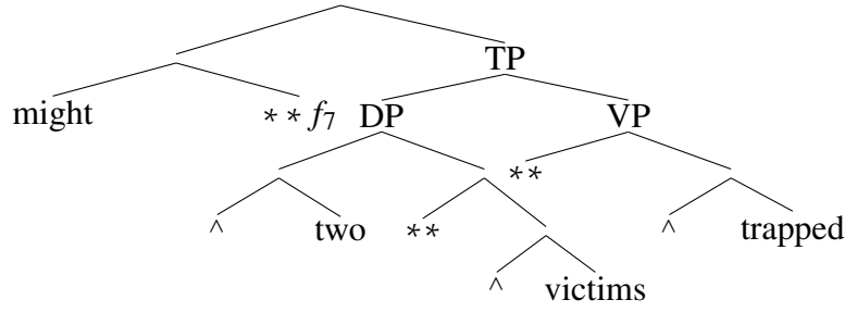
Figure 5 LF that derives R4 for (15), in Keshet’s scope system
