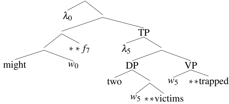
Figure 4 LF that derives R4 for (15), with world variable
